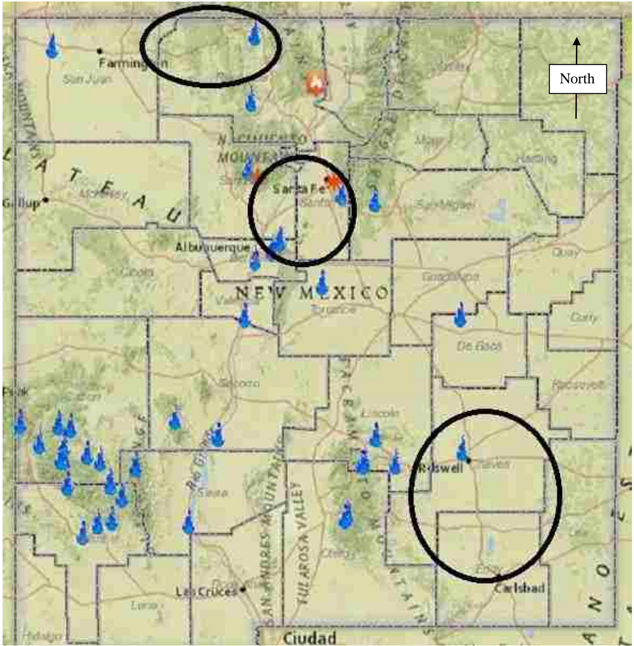
Figure 8: Active and Inactive wildfires in New Mexico
