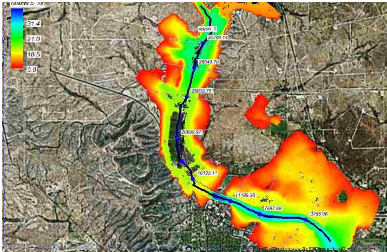
Figure 37: Case III Dam Flood - 75% drainage burnt
